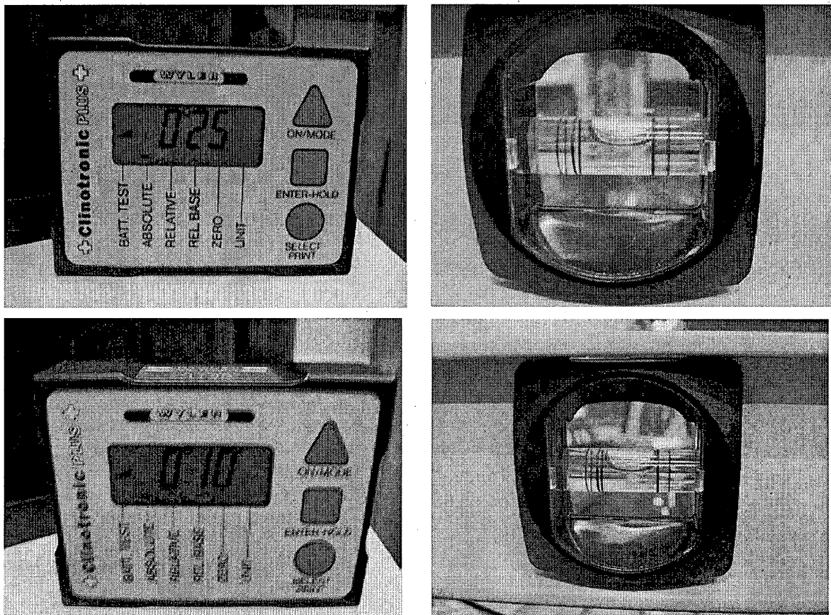
Figure 1 – Comparison of inclinometer and spirit level
